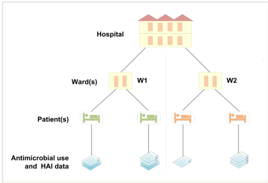
Figure 2: Data hierarchy
