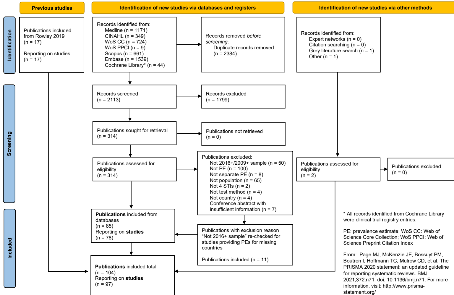
Figure A1. PRISMA flow diagram
